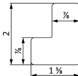
SS FLAT ST FRAME
